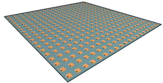
Patch array: 20 x 20 element S-band SAR patch array. Modelled using FDS in 22 minutes using 42 GB RAM on an Intel Core i9-13900K.
