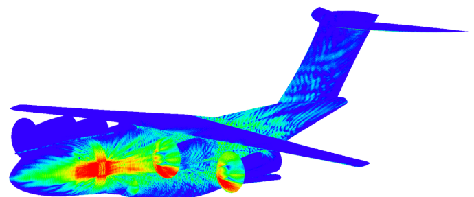
Installed performance: 20 x 20 element S-band SAR array mounted on Airbus A400M. Time: 51 min. RAM: 92 GB on an Intel Core i9-13900K.
