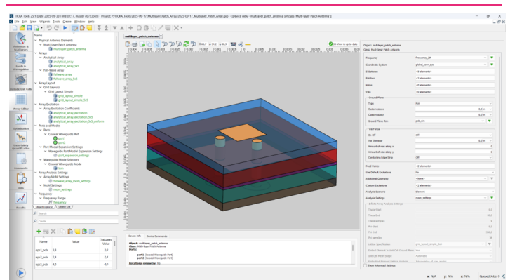
Multi-layer patch: The element wizard makes it easy to set up single- or multilayer patches.
